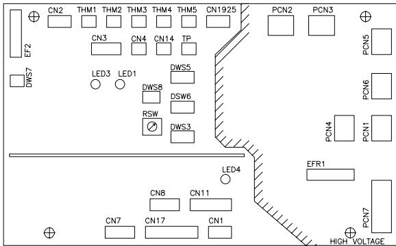
Leiterplatte (Printed Circuit Board)
