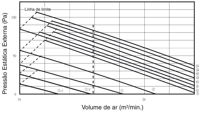
S-60PN1E5 ,S-71PN1E5 Diagrama P-Q
