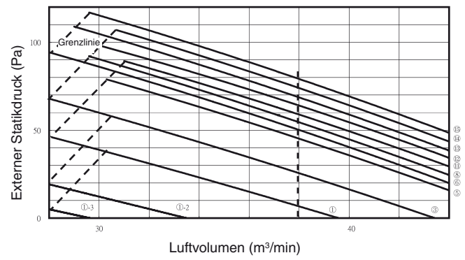
S-125PN1E5 P-Q Diagramm
