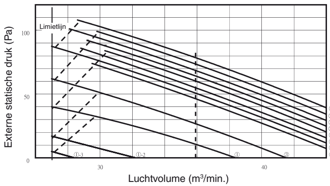
S-100PN1E5 P-Q-diagram
