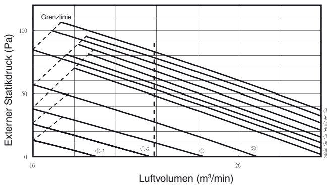
S-60PN1E5 ,S-71PN1E5 P-Q Diagramm
