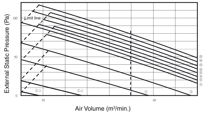
S-125PN1E5 P-Q diagram
