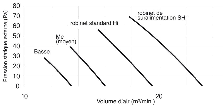
S-45PN1E5, S-50PN1E5 COURBE P-Q
