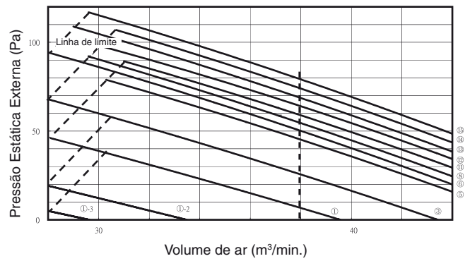
S-125PN1E5 Diagrama P-Q
