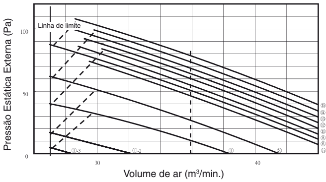
S-100PN1E5 Diagrama P-Q
