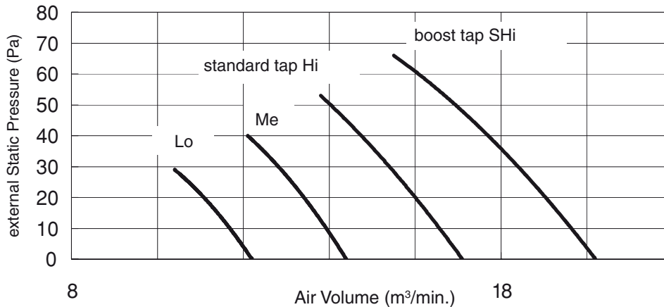
S-36PN1E5 P-Q CURVE
