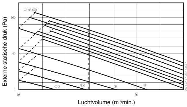
S-60PN1E5 ,S-71PN1E5 P-Q-diagram
