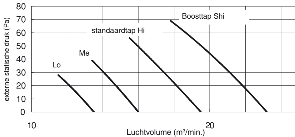
S-45PN1E5, S-50PN1E5 P-Q CURVE
