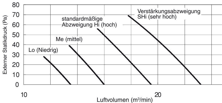
S-45PN1E5, S-50PN1E5 P-Q-KURVE
