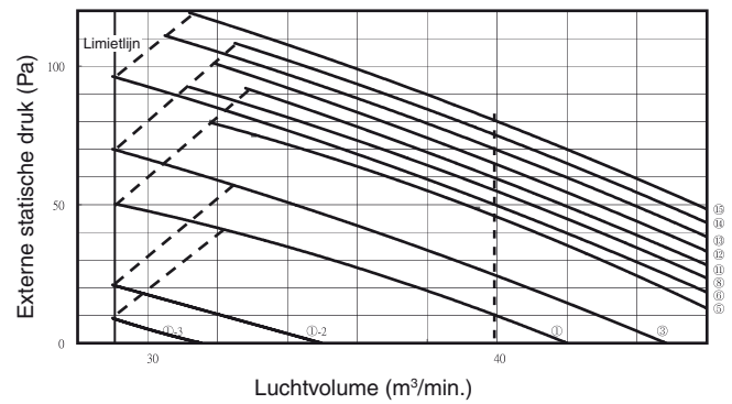
S-140PN1E5 P-Q-diagram
