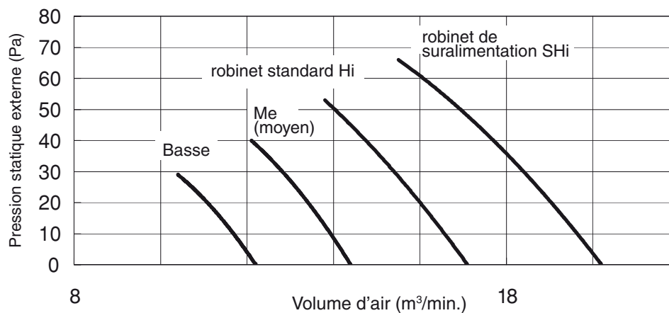
S-36PN1E5 COURBE P-Q
