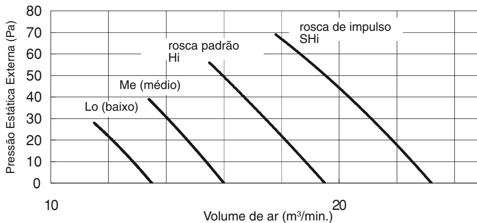
S-45PN1E5, S-50PN1E5 CURVA P-Q
