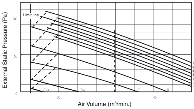
S-100PN1E5 P-Q diagram
