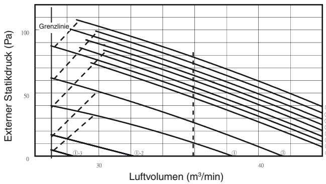
S-100PN1E5 P-Q Diagramm
