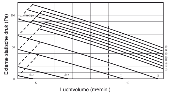
S-125PN1E5 P-Q-diagram
