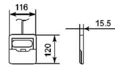
Wired remote control CZ-RD513C
