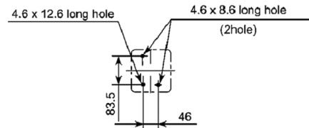
Wired remote control attachment hole position
