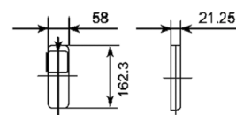
Wireless remote control CZ-RL513B
