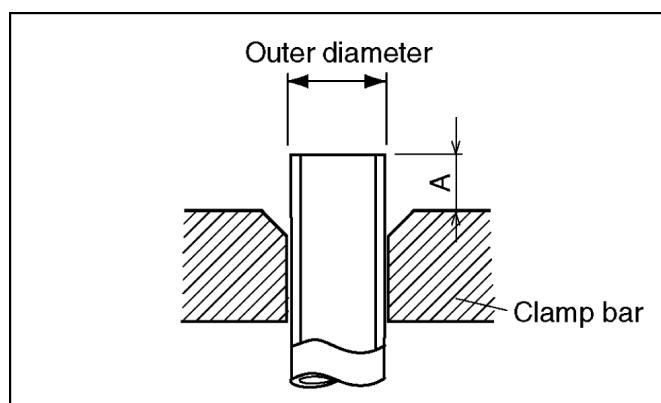
Fig. 10 Flaring dimensions
