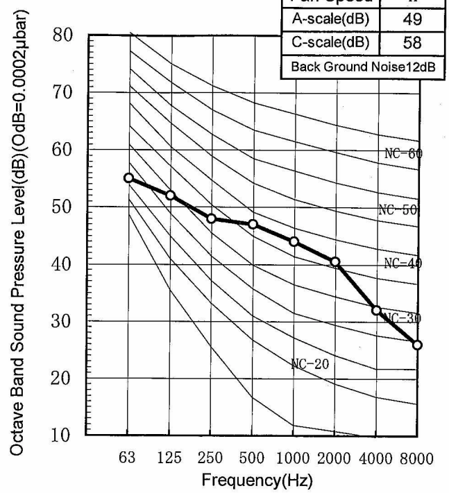
CU-L28DBE5 (Heating) Octave Band Central Frequency(Hz)
