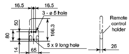
Wireless remote control holder attachment hole position
