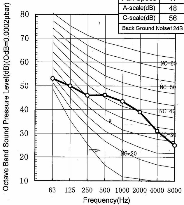
CU-L28DBE5(Cooling) Octave Band Central Frequency(Hz)
