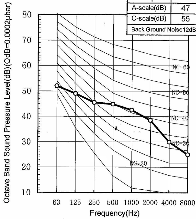
CU-L24DBE5(Cooling) Octave Band Central Frequency(Hz)
