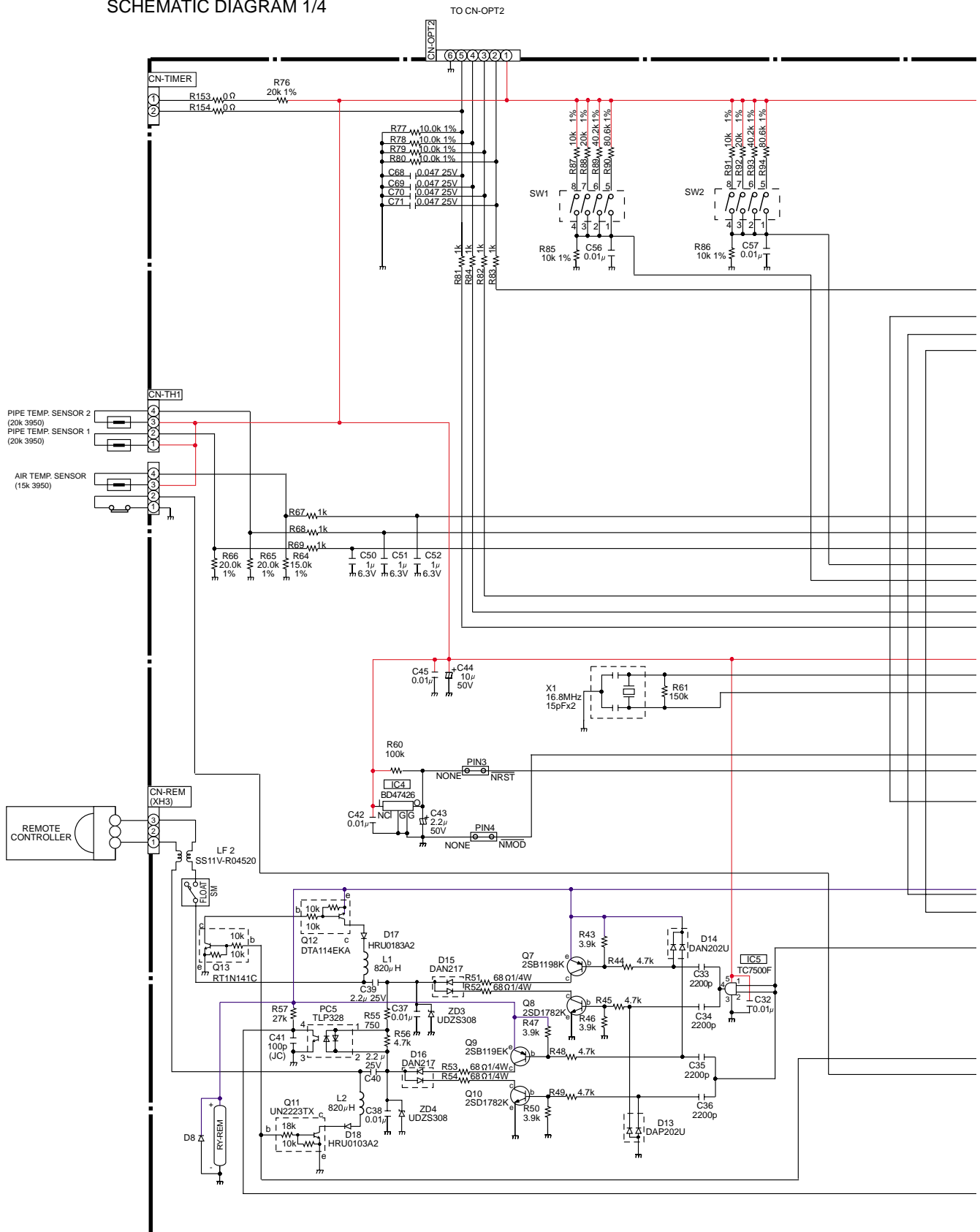
SCHEMATIC DIAGRAM 1/4
