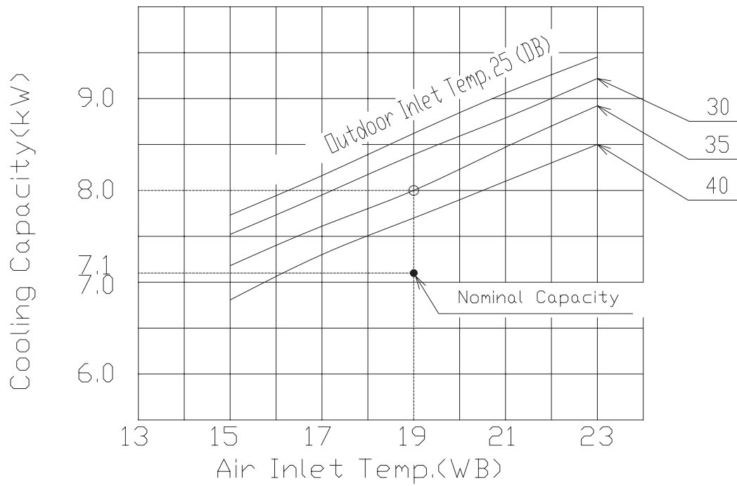
Cooling Capacity curves
