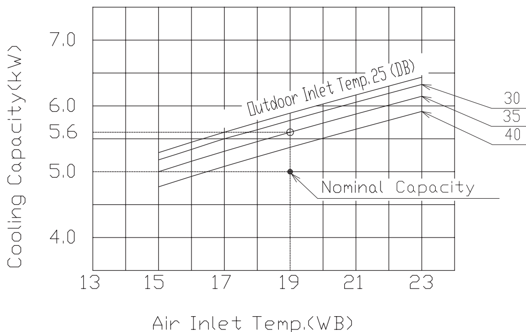
Cooling Capacity curves
