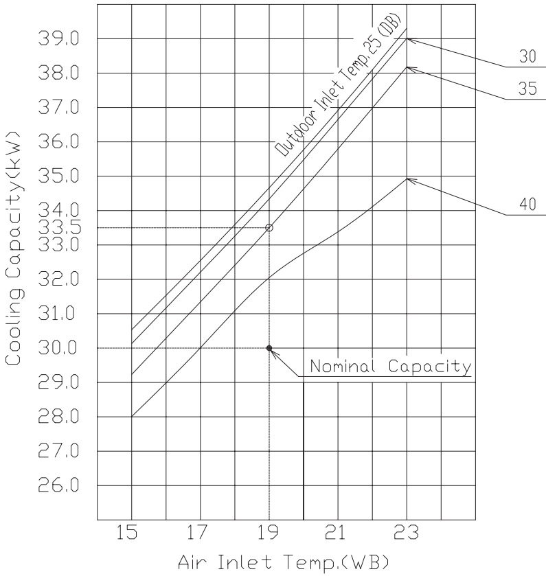
Cooling Capacity curves
