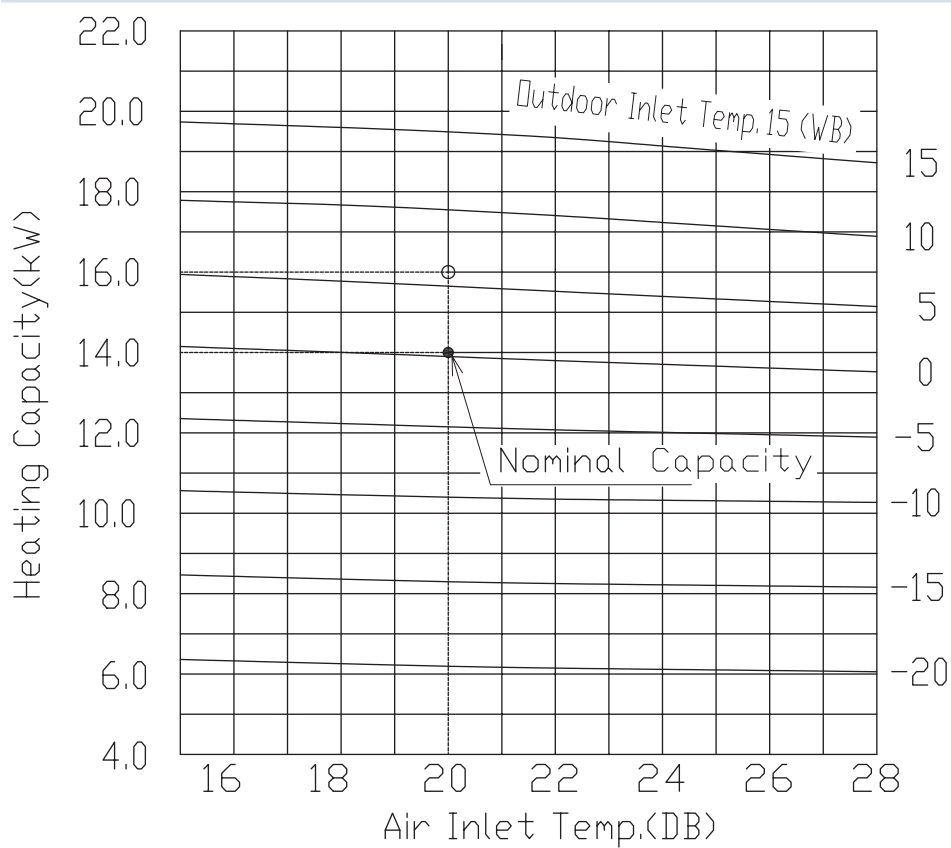
Heating Capacity curves
