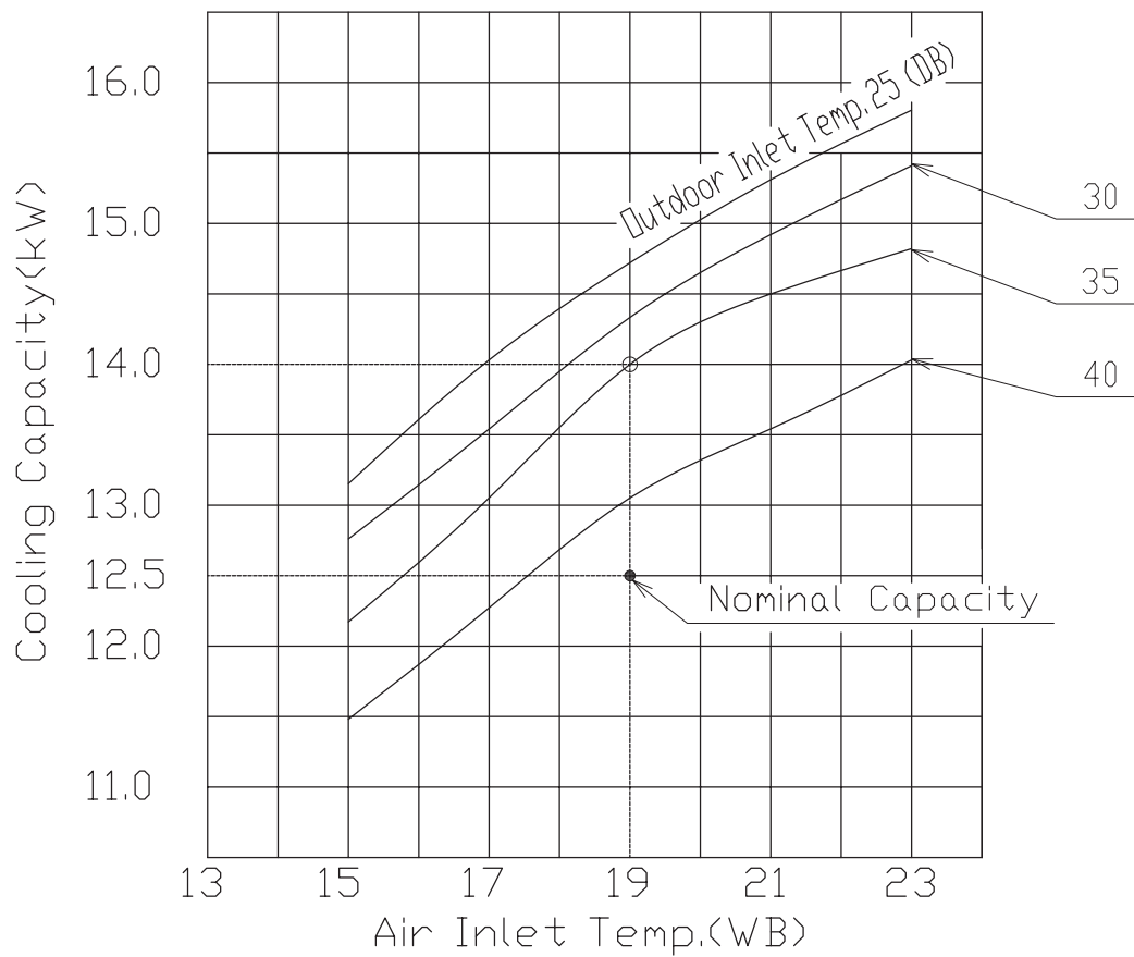
Cooling Capacity curves
