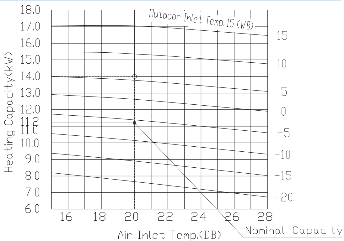
Heating Capacity curves
