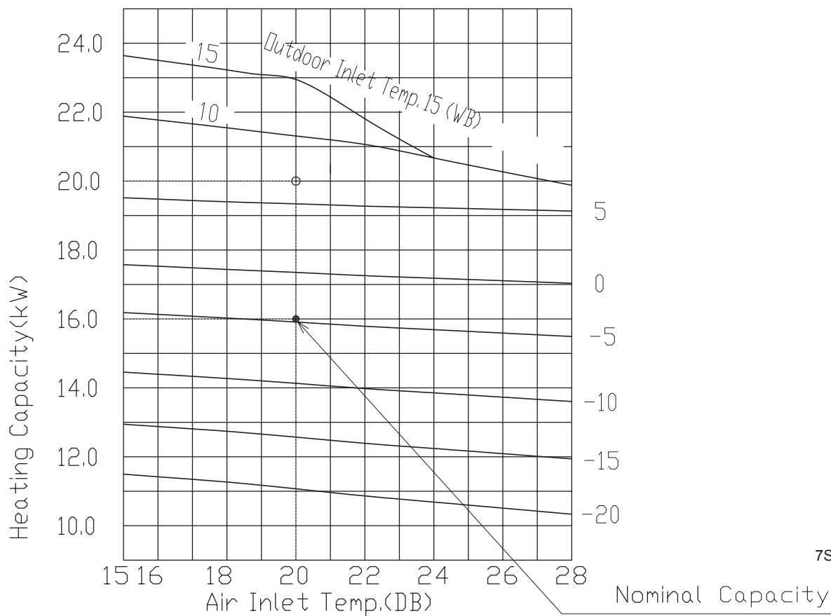
Heating Capacity curves
