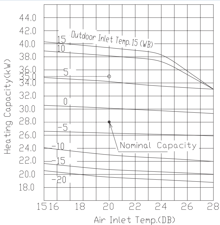
Heating Capacity curves
