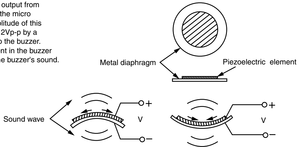
Fig.7-2 Buzzer Operation
