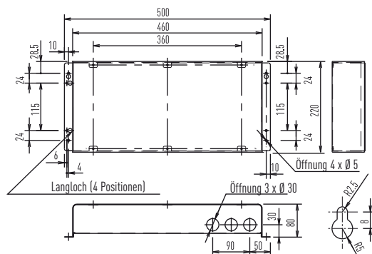
LonWorks-Interface (CZ-CLNC2)
